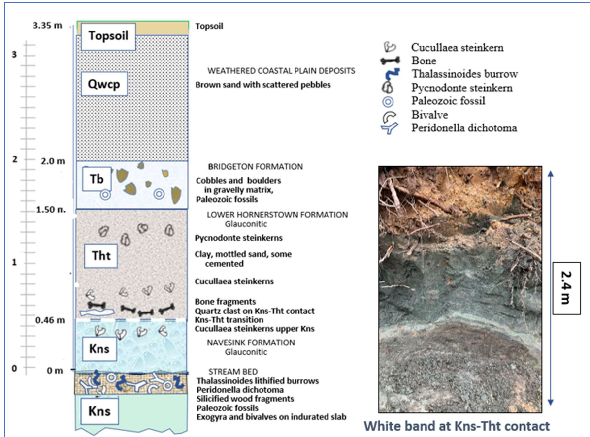
Figure 4. Stratigraphic Section B Turtle Creek site. See site profile Figure 3 for location. The white band at the Kns-Tht contact ranges from 10 cm to 46 cm in width. The bones were recovered from the thicker section of this band off to the right. Sketch by author, MS Word. Photograph by author.
