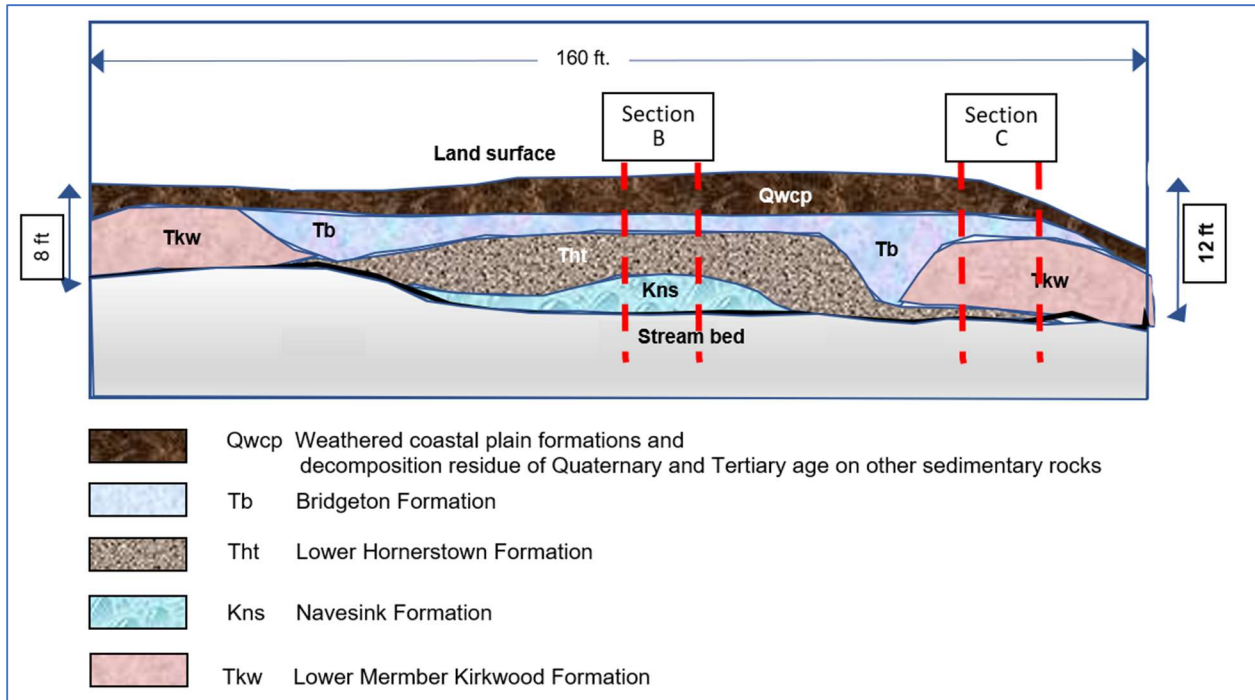
Figure 3. Subsurface geology profile sketched as interpreted along the east bank of the Turtle Creek site, downstream to the right. Sketch by author, MS Word.
