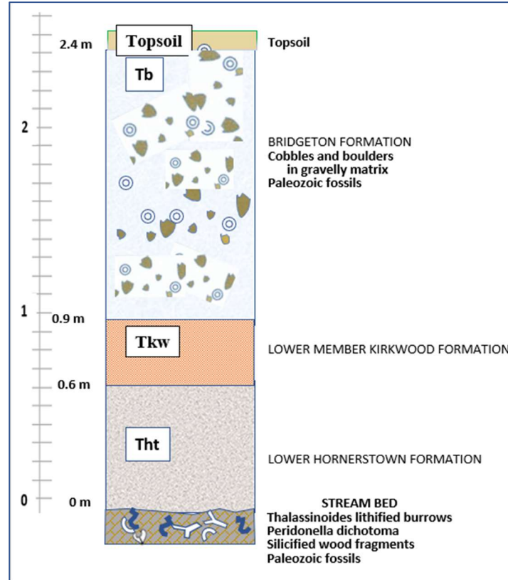
Figure 5. Stratigraphic Section C, showing the layer of Kirkwood Formation, Turtle Creek site. See site profile Figure 3 for location of this section. Sketch by author, MS Word.
