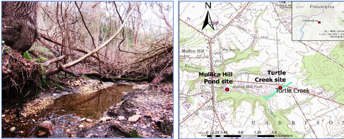
Figure 1. Left. Typical stretch of Turtle Creek showing boulders, cobbles and gravel in the stream bed from which most of the fossils were recovered. View is upstream with formation exposures on the right (east) bank. Photograph by author. Right, Location section of USGS topographic map of the Turtle Creek site relative to the more familiar classic Mullica Hill Pond site. Turtle Creek is highlighted. The Rowan University Edelman Fossil Park site (former Inversand) is off the map to the right. ArcGIS map by author.
