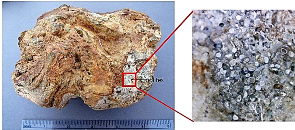
Figure 6. Indurated Mollusca slab from stream bed at Section B, Figure 4 with interior oolites. Photographs by author.
