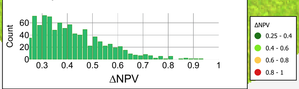
Severity distribution:
