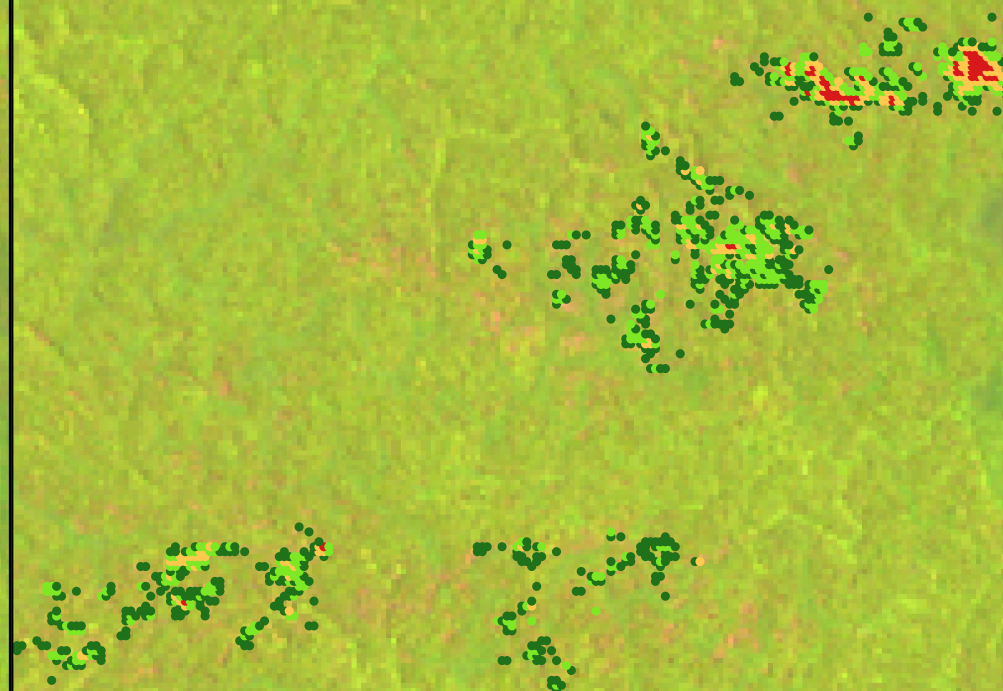
Severity distribution:
