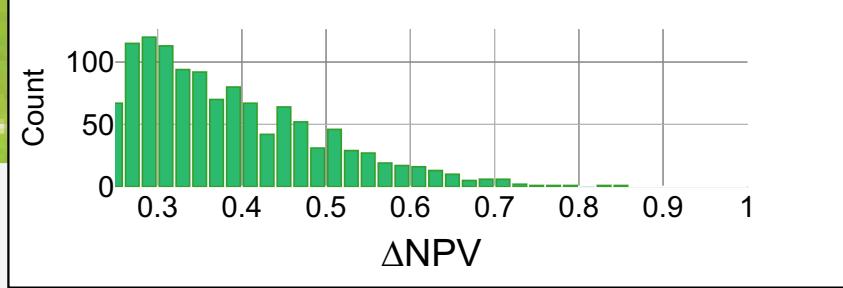
Severity distribution:
