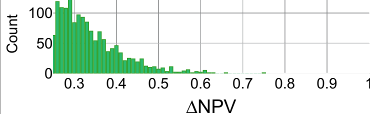
Severity distribution:
