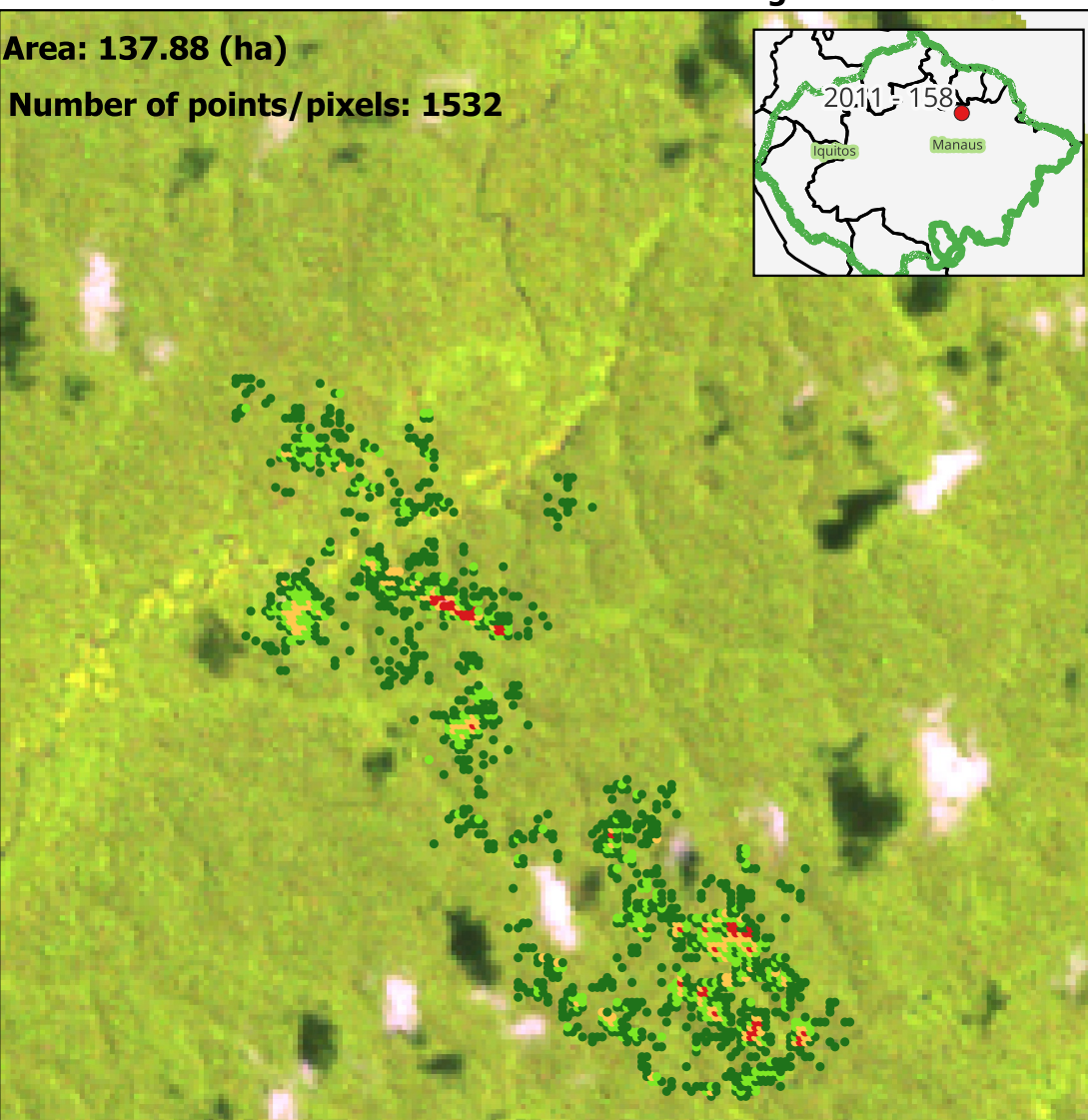
Severity distribution:
