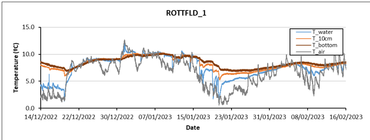
Figure 21. Temperature time series in water, sediment-bed (bottom and 10-cm level), soil and air for field measurements at locations DELTFLD_1 (top) and ROTTFLD_1 (bottom).
