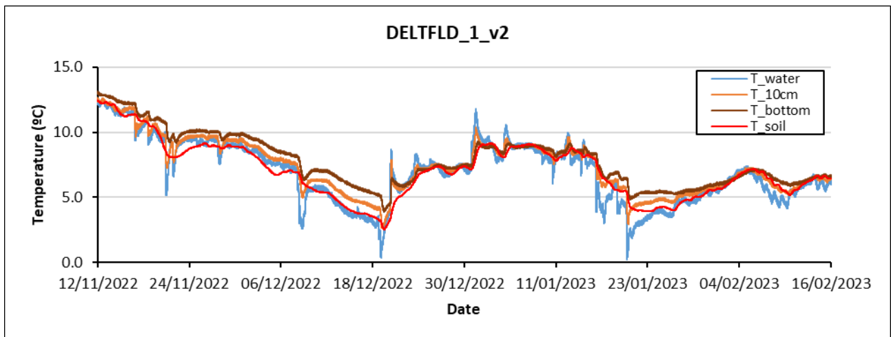
Figure 20. Temperature time series in water and sediment-bed (bottom and 10-cm level) for tests on sand (top), organic (middle) and mix (bottom) sediments; temperature gradients dT1 (left) and dT2 (right); and hydrograph with peak flow at 10 min.
