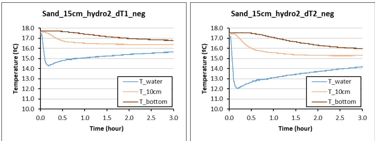
Figures 20 and 21 plot processed temperatures for several laboratory tests and field campaign measurements.
