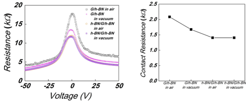
Fig. 3 (a) shows graphene device resistance versus backgate voltage (b) shows the contact resistance for all the cases (G/h-BN on air, G/h-BN in vacuum, h-BN/G/h-BN in air, h-BN/G/h-BN in vacuum)
