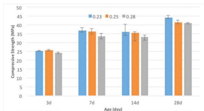
Fig. 5 Effect of water content on the compressive strength of geopolymer mortar
