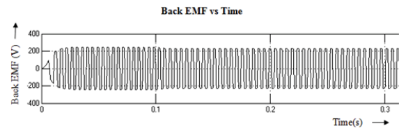
Fig. 14 Back EMF Waveform
