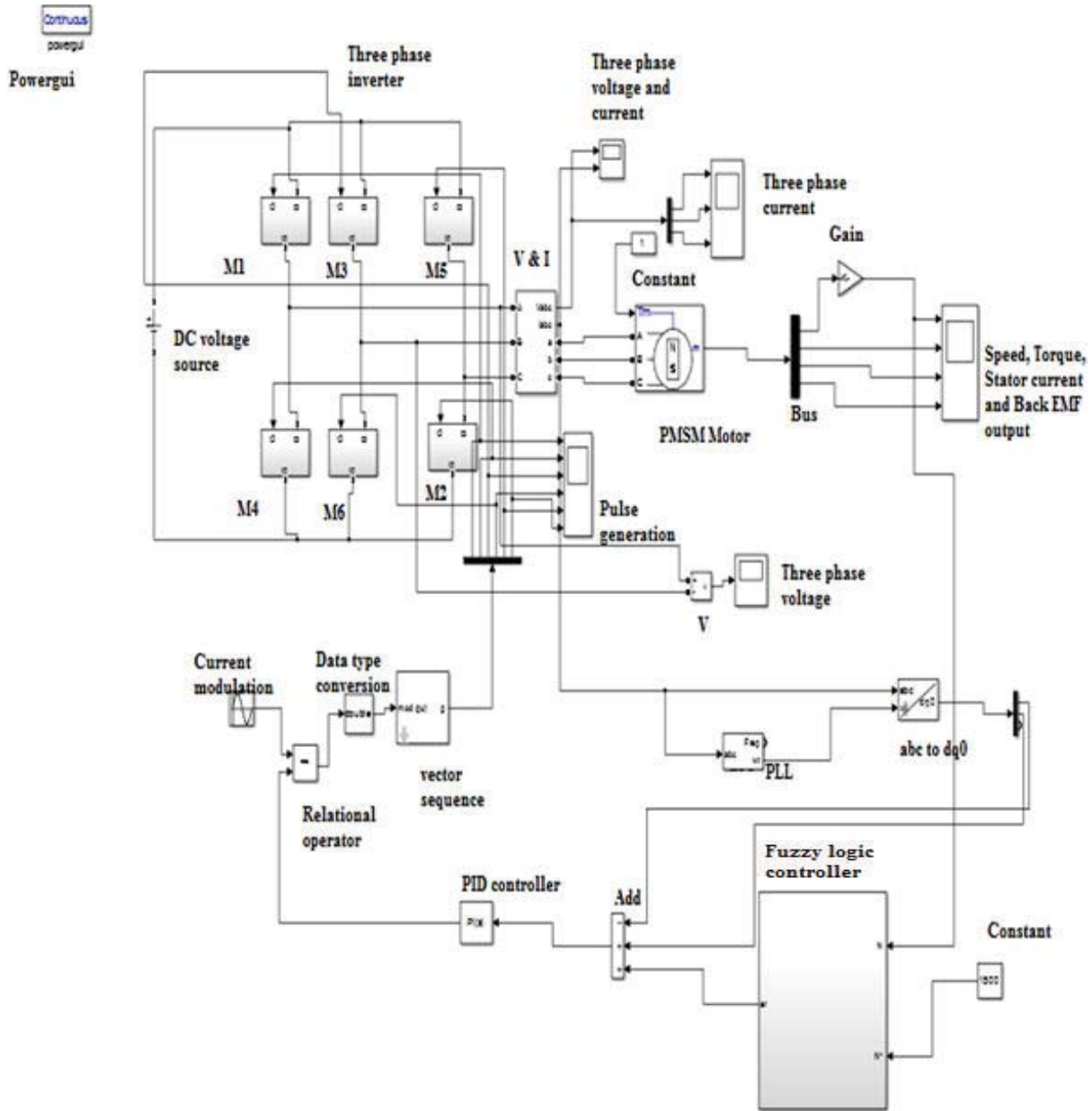
Fig. 5 Simulation Circuit for EA Based Fuzzy PID Controller
