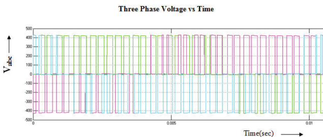
Fig. 11 Waveform for Three Phase Voltage
