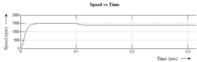
Fig. 12 Speed Waveform for PMSM
