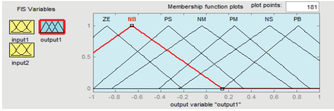
Fig. 8 Membership Function Output
