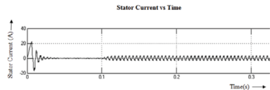
Fig. 15 Waveform for Stator Current
