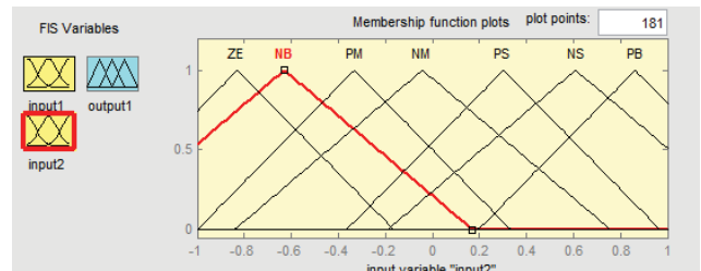
Fig. 7 Membership Function Value for Input 2
