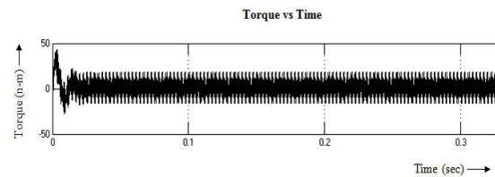
Fig. 13 Torque Waveform for PMSM
