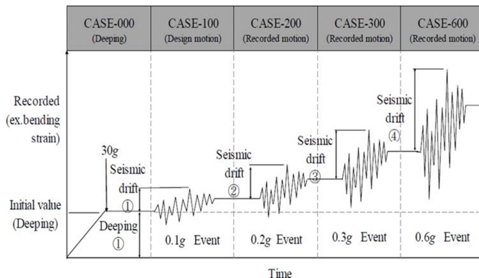
Fig. 4 Reference case testing procedure, as reported in [10]
