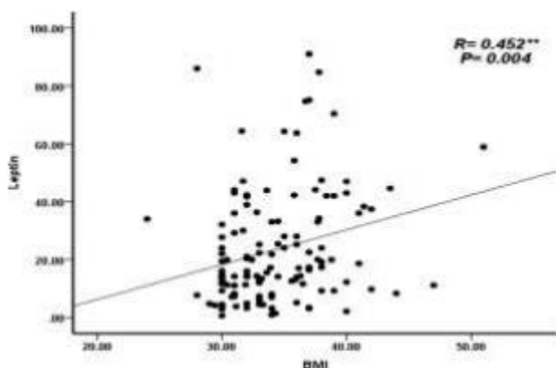
Fig [4]: correlation between BMI and Leptin in obese subjects.
