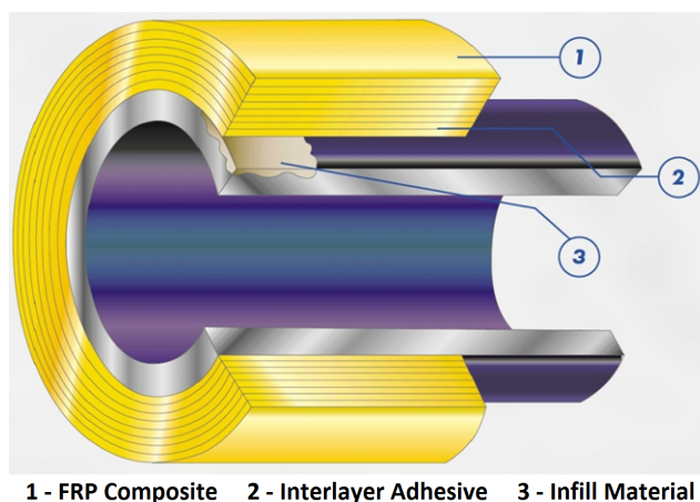
Fig. 2 Clock Spring ® FRP composite repair system
