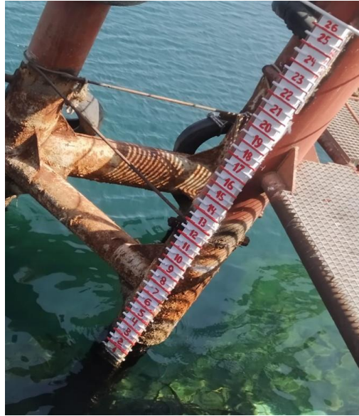
Figure 2. Tamasa is used to measure the water level at the Sea Hydrometeorological Station of the “Neft dashları” in the Caspian Sea
