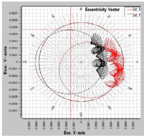
Fig. 7 Violation of the "Normal_vs_Radial separation" circle
