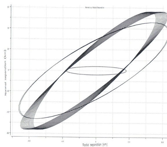
Fig. 9 Two Cases of circle violation for Satellite X, Y
