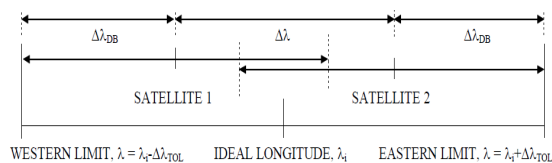
Fig. 2 EW Dead band for longitude Separation Strategy; 2\Delta\lambda_{TOL} = \Delta\lambda + 2\Delta\lambda_{DB} , \Delta\lambda is the separation between satellites
