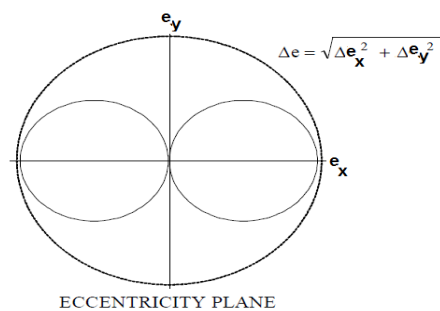
Fig. 3 EW Dead band for Eccentricity Separation Strategy
