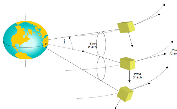
Fig. 6 Satellite pointing in inclined orbit configuration
