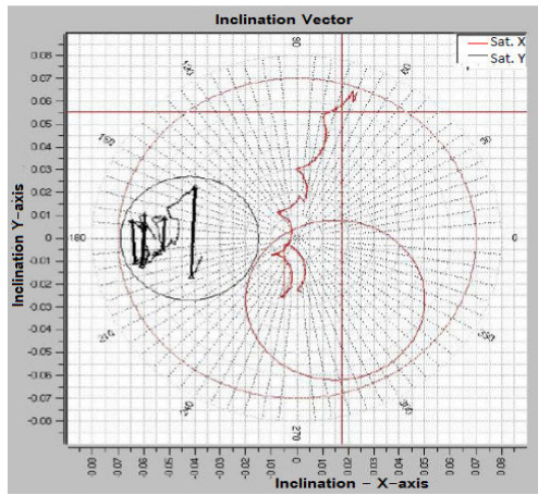
Fig. 7 Violation of the "Normal_vs_Radial separation" circle
