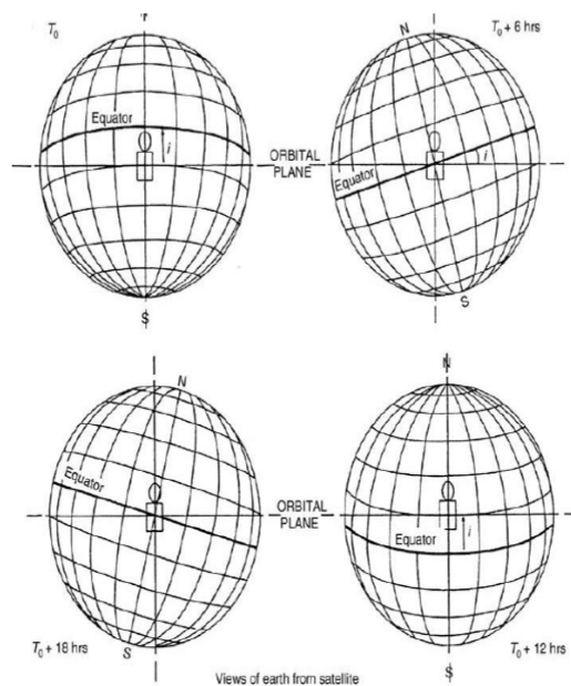
Fig. 5 Satellite inclination-induced Yaw Variation along the orbit
