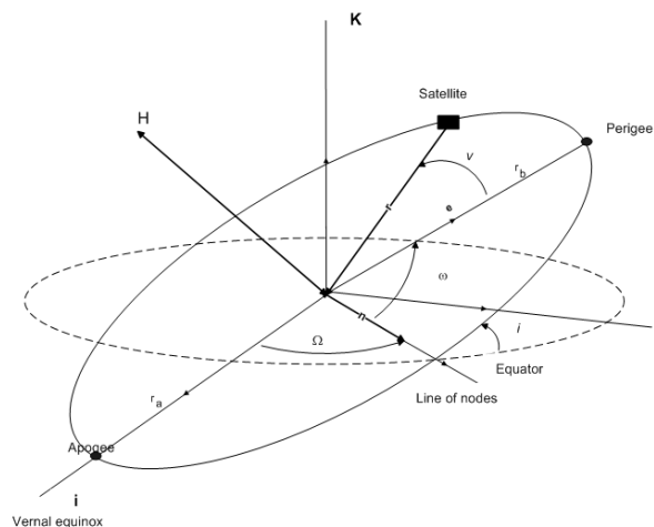
Fig. 1 Orbital angles
