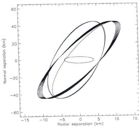
Fig. 9 Two Cases of circle violation for Satellite X, Y
