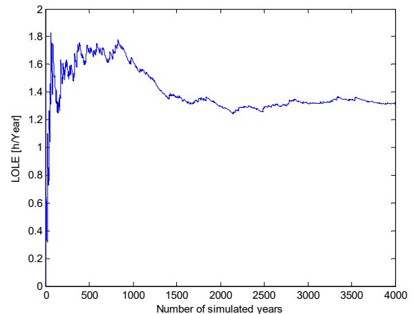
Fig. 2 Illustration of the convergence of the Monte Carlo process for NS = 4000 (evolution of the adjusted LOLE index in the entirely correlated scenario)
