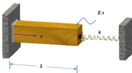
Fig. 2 Cantilever with Fixed Spring
