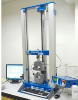
Fig. 8 Tensile strength testing device –Inspekt Desk 5 kN
