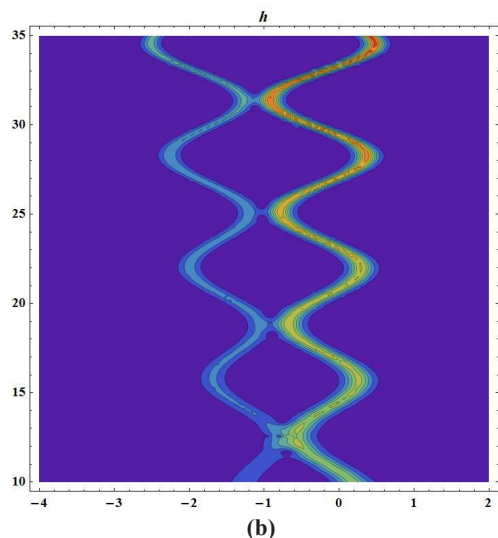
Fig. 1 (a) Intensity profile of two solitons solutions. The parameters are \eta_1 = -0.4, \eta_2 = -0.4, \xi_1 = -0.25, \xi_2 = 0.4, \sigma = 0.05 (b) Corresponding contour plot
