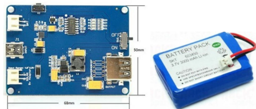
Fig. 11 Energy shield and 7v Lipo battery
