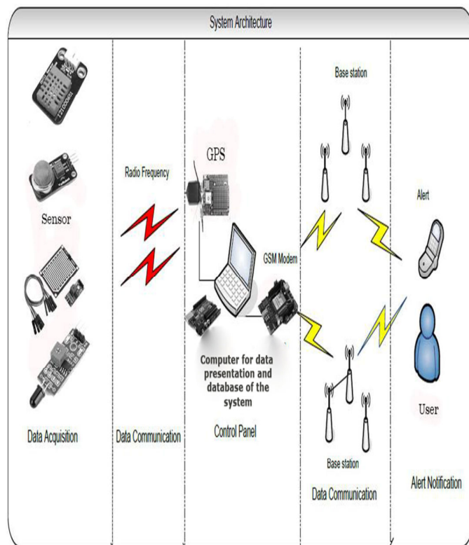
Fig. 3 System architecture
