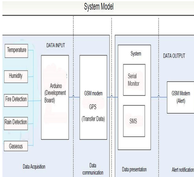
Fig. 2 System model
