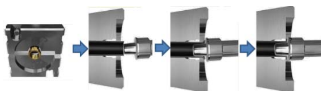
Fig. 2 Orbital-forming process
