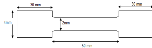
Fig. 4 Dimension for tensile test sample
