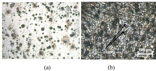
Fig. 12 Micrograph cast sample A2 with 2 mm thick section (a) unetched (b) etched
