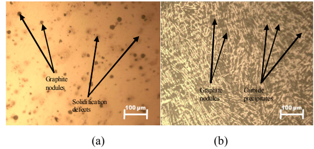
Fig. 9 Micrograph of cast sample A1 with 2 mm thick section (a) unetched (b) etched
