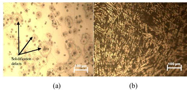
Fig. 11 Micrograph cast sample A1 with 4 mm thick section (a) unetched (b) etched
