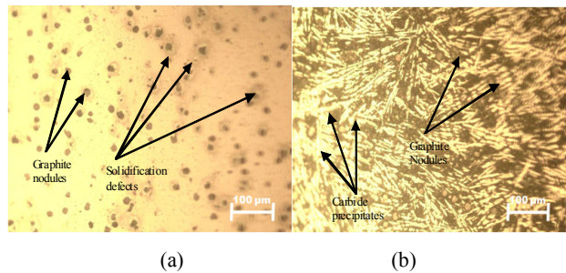
Fig. 10 Micrograph cast sample A1 with 3 mm thick section (a) unetched (b) etched
