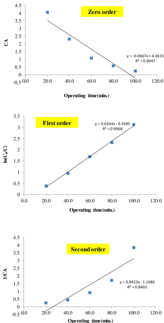
Fig. 6 The zero, first and second orders were plotted C_A , \ln(C_{A0}/C_A) and 1/C_A against time
