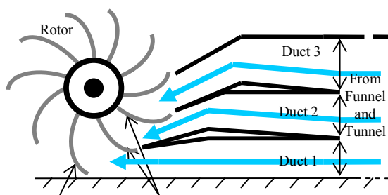
Fig. 5 A variable duct turbine for different wave heights and sea levels
