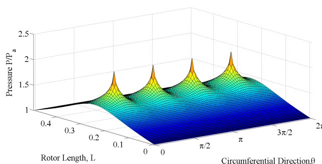
Fig. 6 3D view of pressure distribution at supply pressure 3 atm, eccentricity 0 and radial clearance 75\ \mu\text{m}
