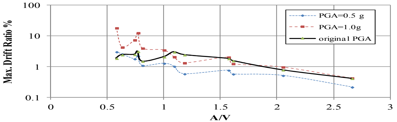
Fig. 7 Variation of maximum inter-story drift ratio with factor A/V, for various PGA
