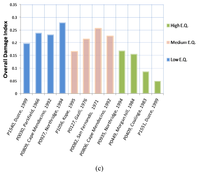
Fig. 4 Overall damage indices of RC building, for EQ having various PGA and frequency contents; Earthquakes are scaled to have PGA=0.5g (a), Earthquakes are scaled to have PGA=1.0g (b), Earthquakes have their original PGA (c)
