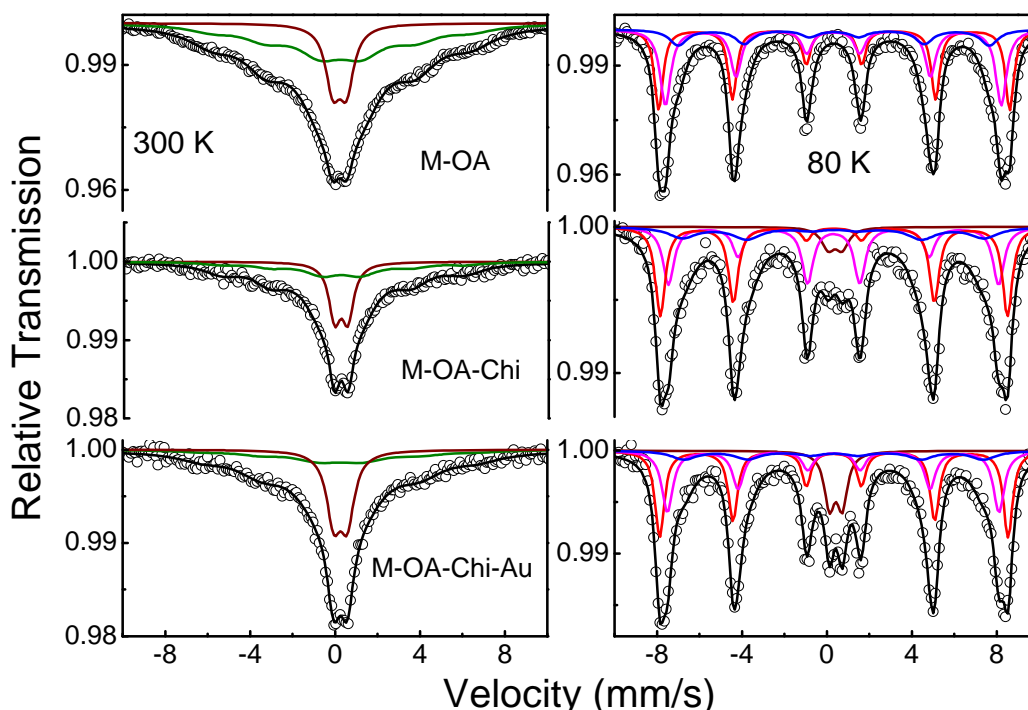
Fig. 4 Mössbauer spectra of oleic acid coated Fe 3 O 4 , Chitosan functionalized Fe 3 O 4 and Chitosan functionalized Fe 3 O 4 @Au core shell nanoparticles at 300 and 80K
