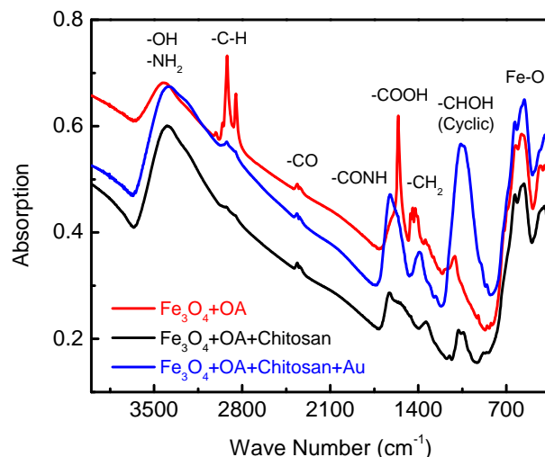
Fig. 3 FTIR spectra of oleic acid coated Fe 3 O 4 , Chitosan functionalized Fe 3 O 4 and Chitosan functionalized Fe 3 O 4 @Au core shell nanoparticles
