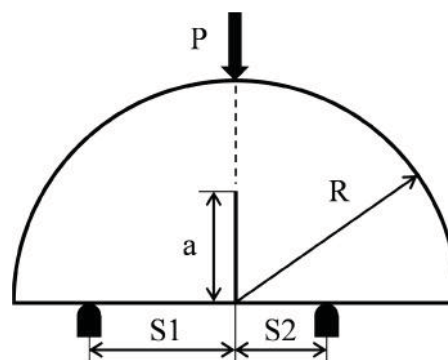
Fig. 2 Semi-circular specimen subjected to three-point bend loading
