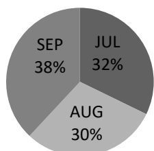
Figure 6: Wet/Rainy Season RH in Percentage Variation
