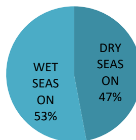
Figure 8: Overall Average Dry and Wet/Rainy Season PM 2.5 in Percentage Variation
