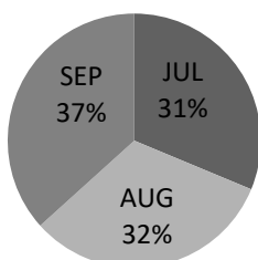
Figure 4: Wet/rainy Season Pm10 in Percentage Variation
