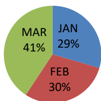
Figure 3: Dry Season RH in Percentage Variation
