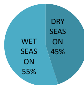
Figure 9: Overall Average Dry and Wet/Rainy Season RH in Percentage Variation
