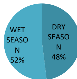
Figure 7: Overall Average Dry and Wet/Rainy Season PM10 in Percentage Variation
