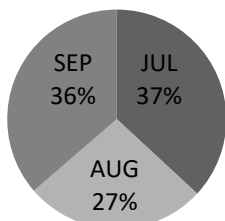
Figure 5: Wet/Rainy Season pm2.5 in Percentage Variation
