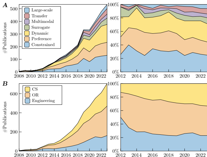
Fig. 11. (Left) Number of publications per year and (Right) relative percentages for (A) the 7 topics on MO variants, (B) the 3 application domains. For the right panel, we truncated the time range to 2012-2023 as the number of publications before 2012 is relatively small.
