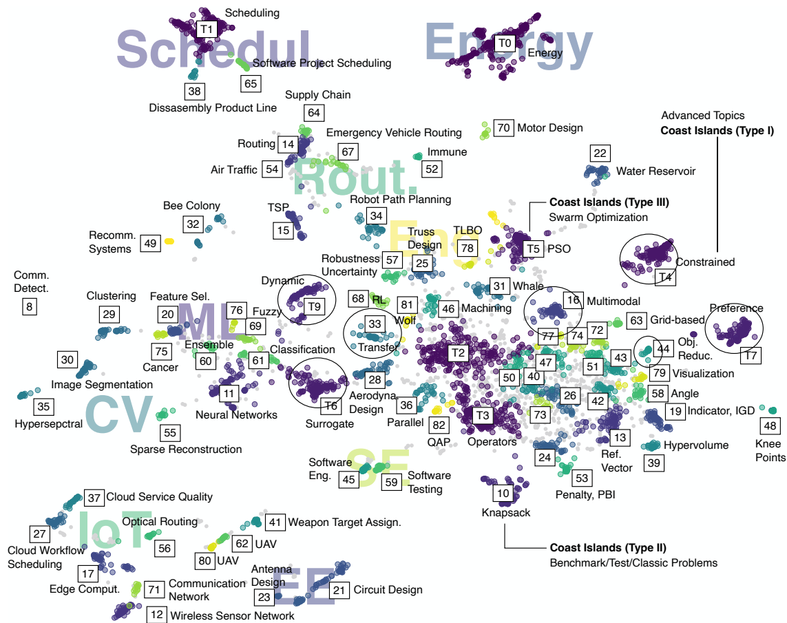
Fig. 8. Low-dimensional visualization of the MOEA/D literature landscape by projecting the paper embeddings using UMAP. Papers are colored and labeled by BERTopic topics. Outliers are shown in light gray. Advanced topics discussed in PART I are circled.
