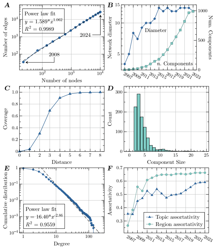
Fig. 19. General patterns for MOEA/D author collaboration networks. (A) Network growth during 2008 and 2024. (B) Network diameter (largest connected component) and number of connected components each year. (C) Percentages of nodes that can be reached within different numbers of hubs from the highest-degree node in the largest connected component. (D) Distribution of the size of the connected components in the network, excluding the largest one. (E) Cumulative distribution of author connections within the network. (F) Assortativity coefficient for author nationality and primary research interest.
