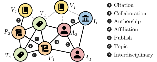
Fig. 2. An illustration of the MOEA/D knowledge graph, containing 5 types of entities and 7 types of relationships.
