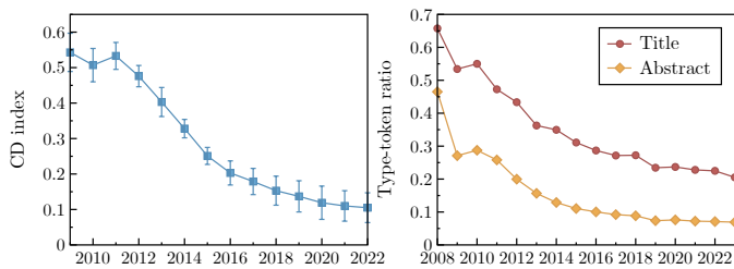
Fig. 15. Paper disruptiveness for MOEA/D literature across time as measured by (Left) the CD index (Right) type-token ratio in paper titles and abstracts. Note that as the calculation of CD index requires information regarding both ancestor and successor papers, the data ranges from 2009 to 2022.
