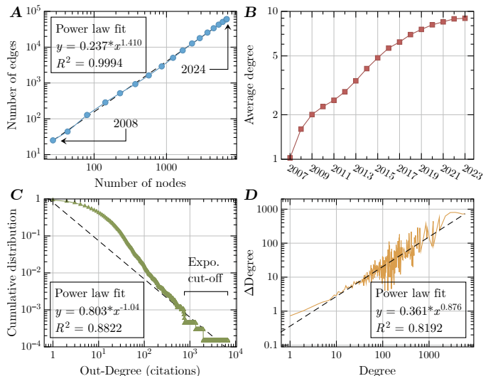
Fig. 14. General patterns for MOEA/D citation networks. (A) The growth of the network nodes and edges from 2008 to 2024. (B) The average degree of the network each year. (C) Cumulative distribution of the number of citations of each paper within the network. (D) The number of new citations of a paper per year as a function of the citation it has already collected.
