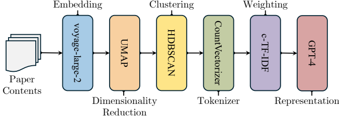
Fig. 6. A high-level overview of the BERTopic framework with our adopted implementations.
