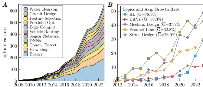
Fig. 12. Number of publications per year for (A) top-10 popular applications topics and (B) top-5 emerging application topics.
