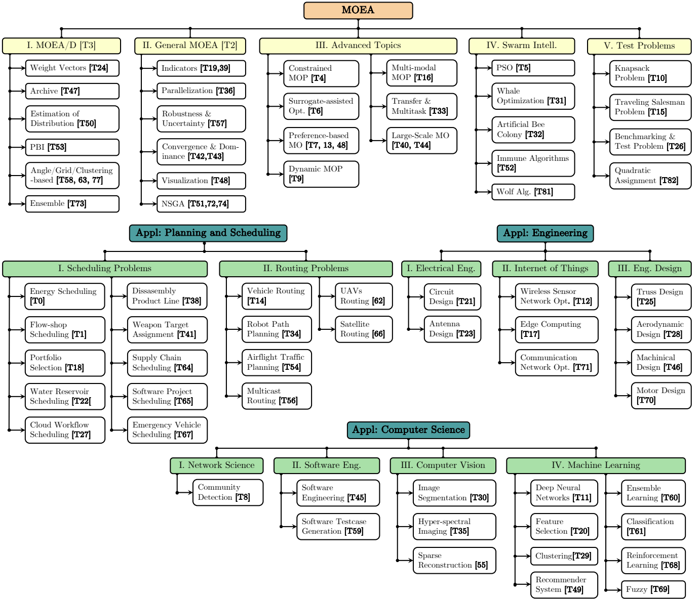
Fig. 7. Hierarchical structure of the BERTopic topics.
