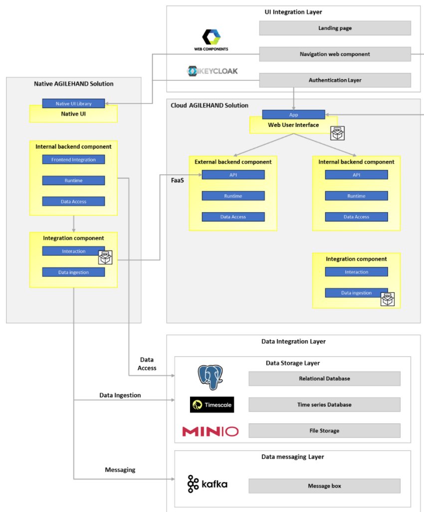
Figure 1: The AGILEHAND solutions architecture.
