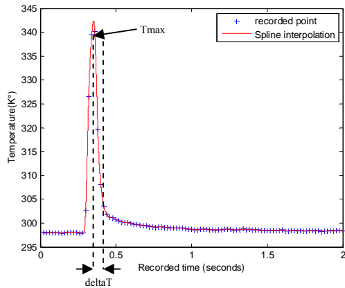
Fig. 5 Temporal variations of the temperatures recorded by the IR camera at the selected X-Y coordinate (dotted line) and temporal variations interpolated by spline (continuous line)
