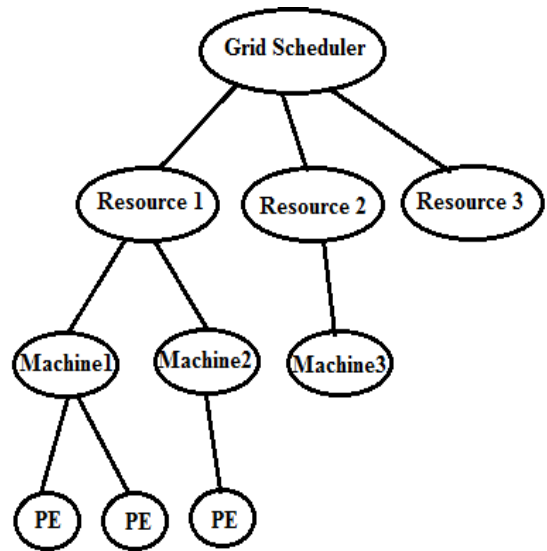
Fig. 3 GridSim Architecture
