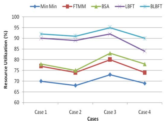
Fig. 7 Performance based on Resource Utilization (%)
