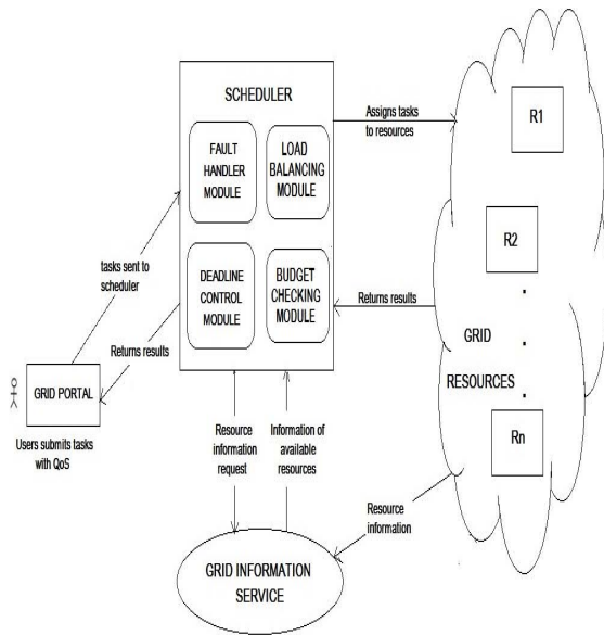
Fig. 2 BLBFT Architecture
