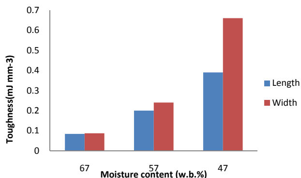
Fig. 17 Effect of moisture and loading orientation on toughness
