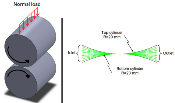
Fig. 2 Schematic view of the CFD model for the cylinders contact problem
