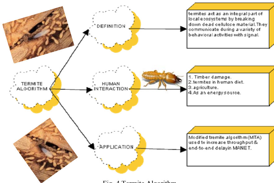
Fig. 4 Termite Algorithm
