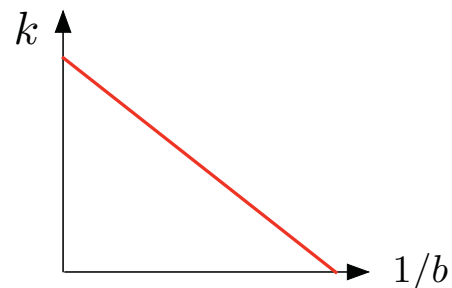
Fig. 2. Bernstein-Goriatchkin model
