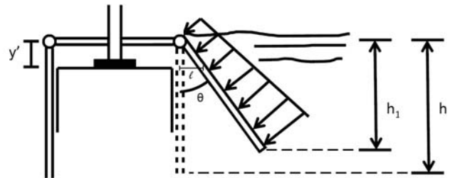
Fig. 12. Calculation of the force exerted by the regolith on the clearing plates
