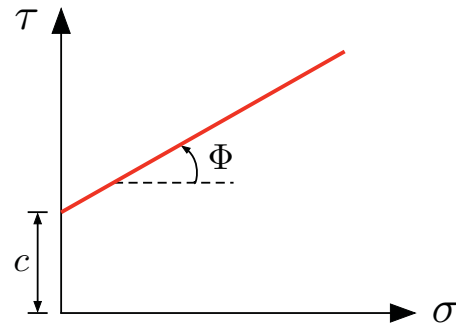
Fig. 1. Mohr-Coulomb failure criterion
