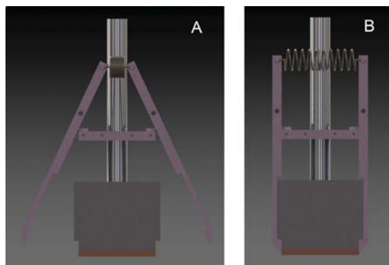
Fig. 7. A: Shearing mechanism from side view (closed) B: Shearing mechanism from side view (open)
