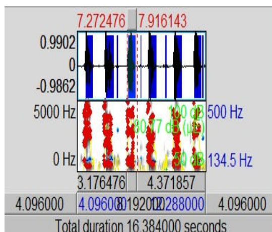
Fig. 1 Speech Sample
