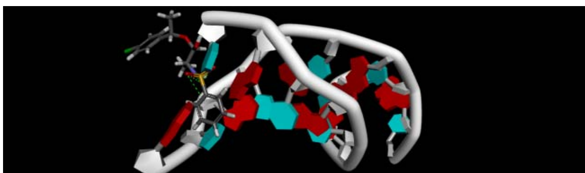
Fig. 4 Docked structure of compound (a) bound to Poly(dA-dT).Poly(dA-dT)
