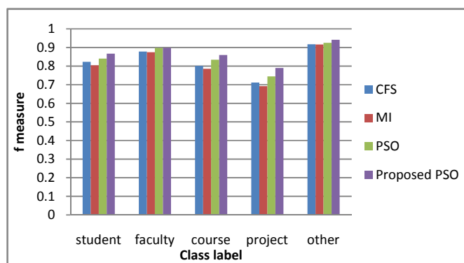
Fig. 5 f measure
