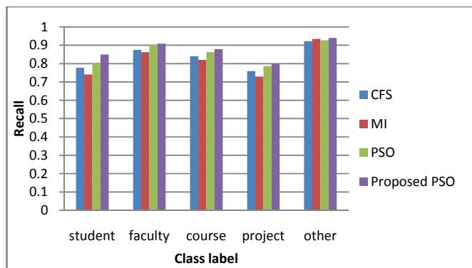
Fig. 4 Recall
