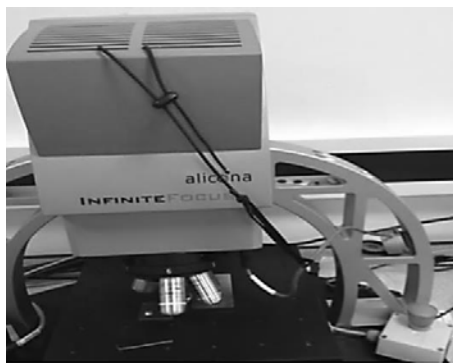
Fig. 10 3D wear measurements using alicona (INFINITE FOCUS)
