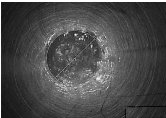
Fig. 7 Pin wear scar diameter using digital microscope
