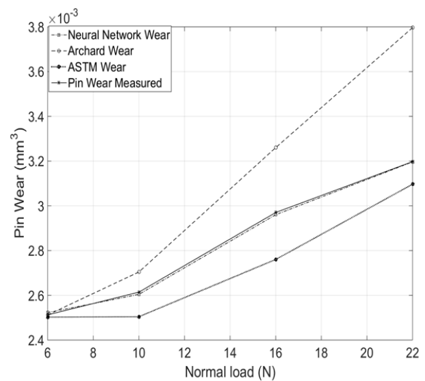
Fig. 13 Pin wear measured, Archard, ASTM, and neural network wear
