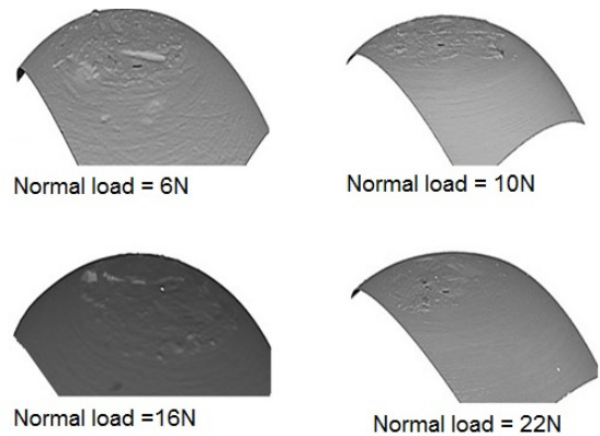
Fig. 12 Pin wear scar measured by using alicona
