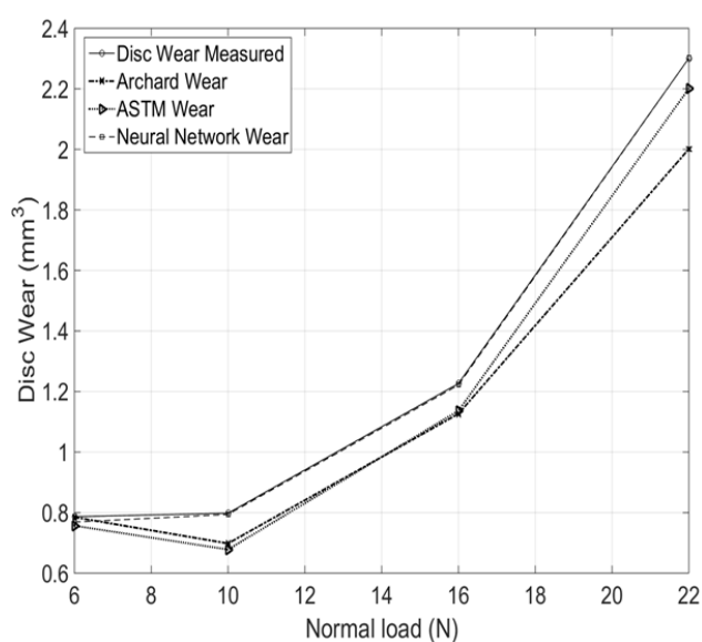
Fig. 14 Disc wear measured, Archard, ASTM, and neural network wear
