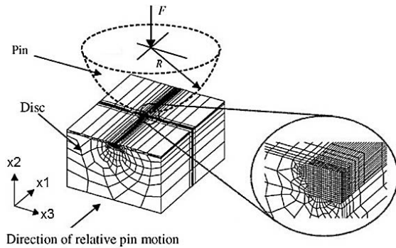
Fig. 9 3D pin/disc contact analysis [13]
