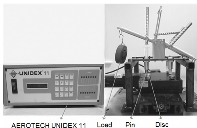
Fig. 1 Pin-on-disc (AEROTECH UNIDEX 11)
