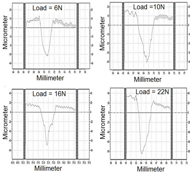
Fig. 3 Disc wear scar depth measured by using Talysurf
