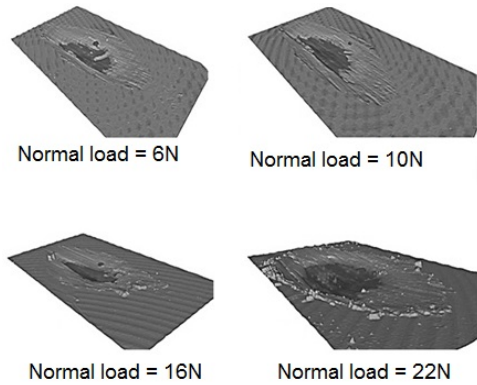
Fig. 11 Disc wear scar measured using alicona
