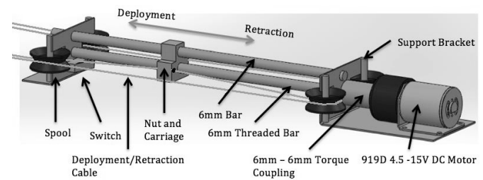
Fig. 7 Drive Mechanism
