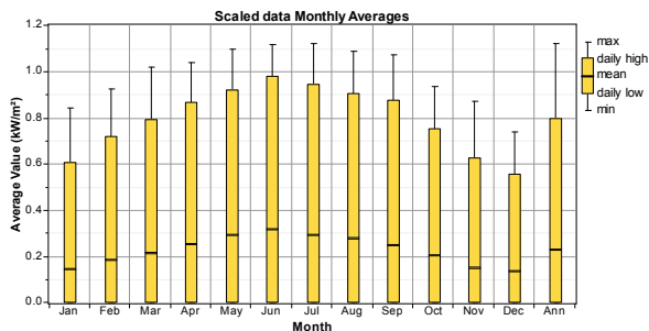
Fig. 9 Monthly average daily solar radiation for South
