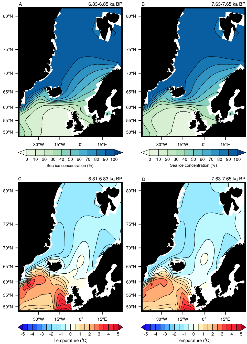
Supplementary Figure 2. Sea-ice concentration in (A) 6.83-6.85 ka BP and (B) 7.63-7.65 ka BP in the TraCE-21ka. Subsurface (92 m) temperature in (C) 6.81-6.83 ka BP and (D) 7.63-7.65 ka BP in the TraCE-21ka.
