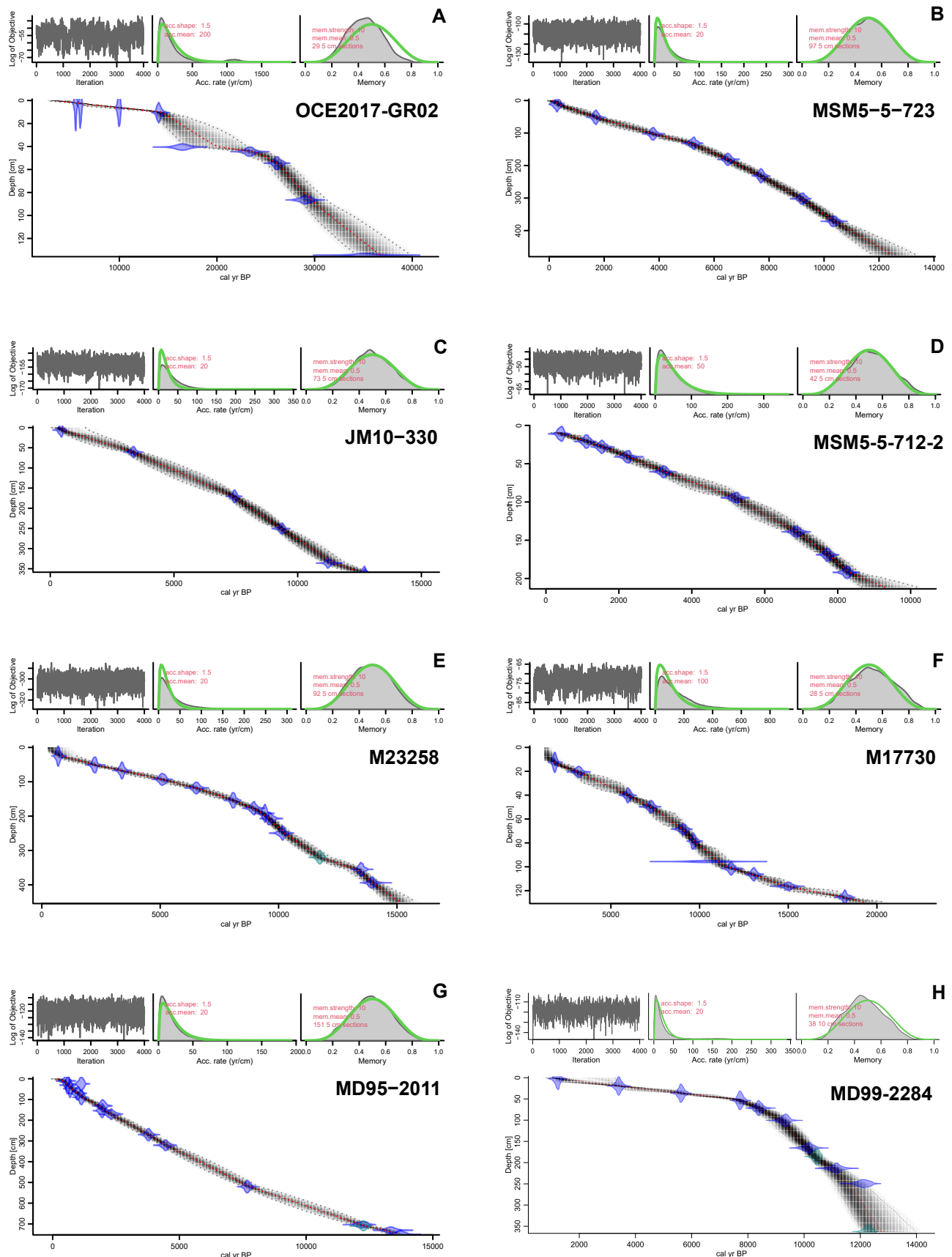
Supplementary Figure 1. Age-depth relationships of cores used in the study as modeled using a Bayesian approach with the Bacon software (Blaauw and Christen, 2011). Dark shading indicates the more likely ages for a given depth, the grey dashed line indicates the 95% confidence range, and the red dashed line indicates the best-fit (mean) age model.
