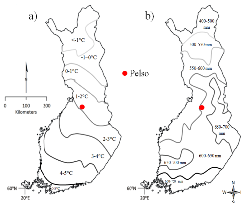
Fig. 1 Study area in Finland's map of (a) average annual temperature ( ^{\circ}\text{C} ) and (b) average annual precipitation (mm), during 1981-2010 Compiled based on [9]
