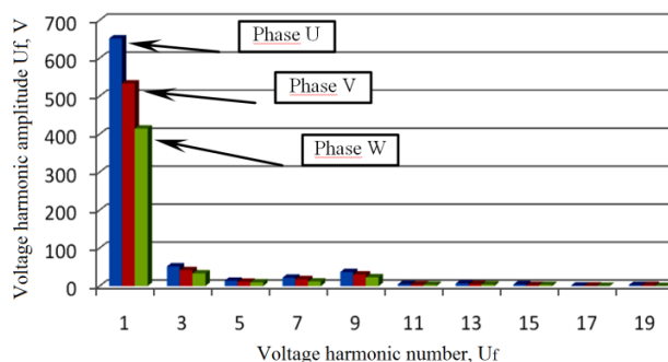
Fig. 7 Spectrum of phase voltage waveforms for each phase of generator in special design
