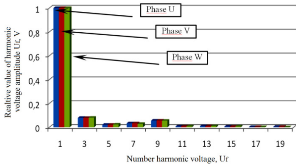
Fig. 8 Spectrum of phase voltage waveforms in relative units for each phase of generator in special design
