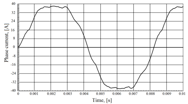
Fig. 12 Calculated waveforms of the phase current in load state of phase U
