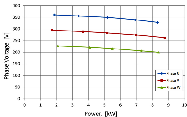
Fig. 22 Measured characteristics of phase voltages vs. power load of each phase of generator for 1000 rpm
