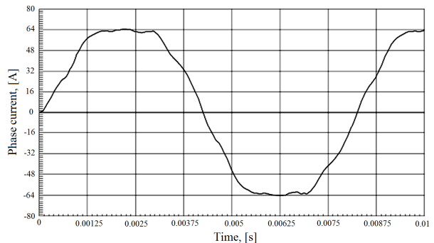
Fig. 14 Calculated waveforms of the phase current in load state of phase W
