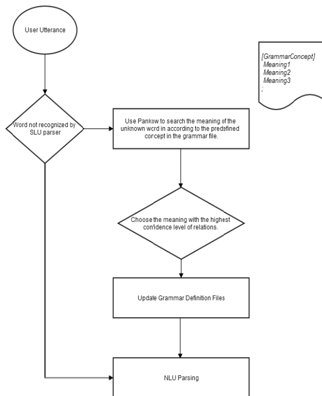
Fig. 1 A self-learning Grammar System Schema
