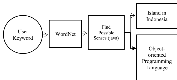
Fig. 4 Identifying different senses of java using WordNet
