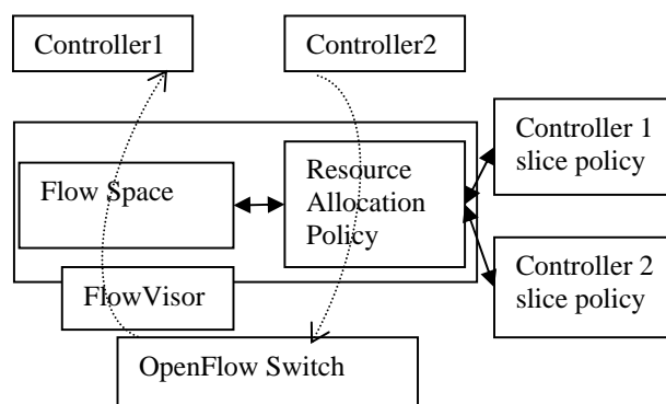
Fig. 1 FlowVisor Architecture [1]
