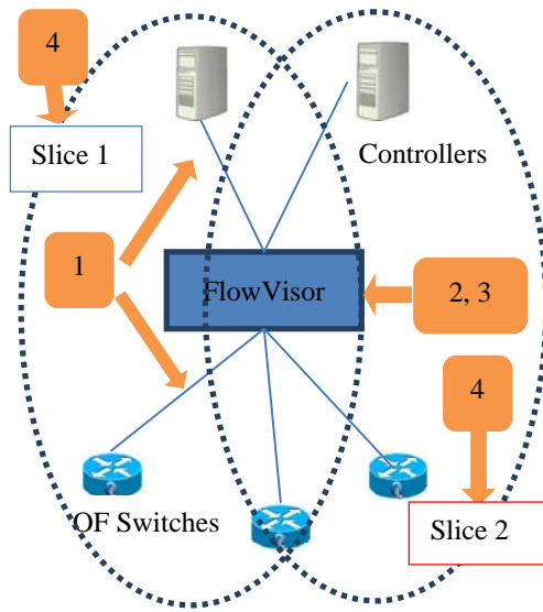
Fig.2 Threats Model
