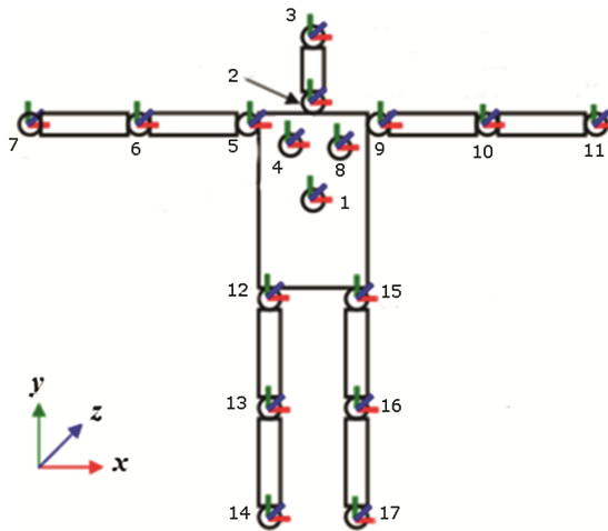
Fig. 3. 17-joint, OpenNI-based hierarchy of control structures defined for REVERIE Kinect Puppetted characters. Joints are identified as follows: (1) Torso; (2) Neck; (3) Head; (4) Left Collar; (5) Left Shoulder; (6) Left Elbow; (7) Left Wrist; (8) Right Collar; (9) Right Shoulder; (10) Right Elbow; (11) Right Wrist; (12) Left Hip; (13) Left Knee; (14) Left Foot; (15) Right Hip; (16) Right Knee; (17) Right Foot.
