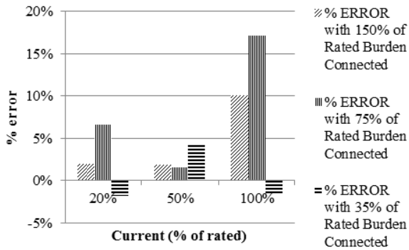
Fig. 1 % Transformation Error for different connected burden
