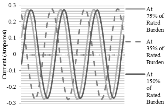
Fig. 2 CT secondary Current waveform when 20% of rated current is injected for different burden
