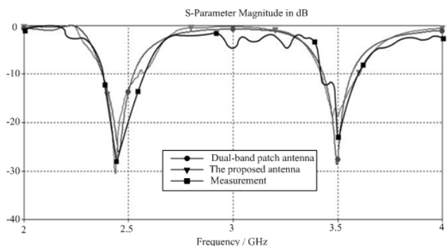
Fig. 9 Comparison of simulation and measurement return loss
