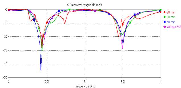
Fig. 7 The S_{11} of dual band antenna
